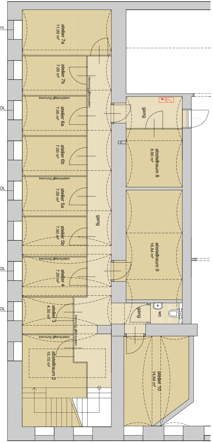
grundriss_ug
